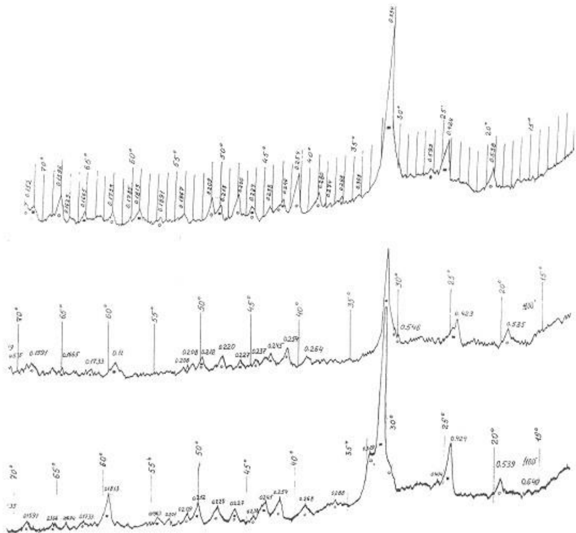
Figure 1. X-Ray Diffraction Patterns Of Samples From Mass C-1, Fired At Different Temperatures, 0c: A) 1100; B) 1200; C) 1250
