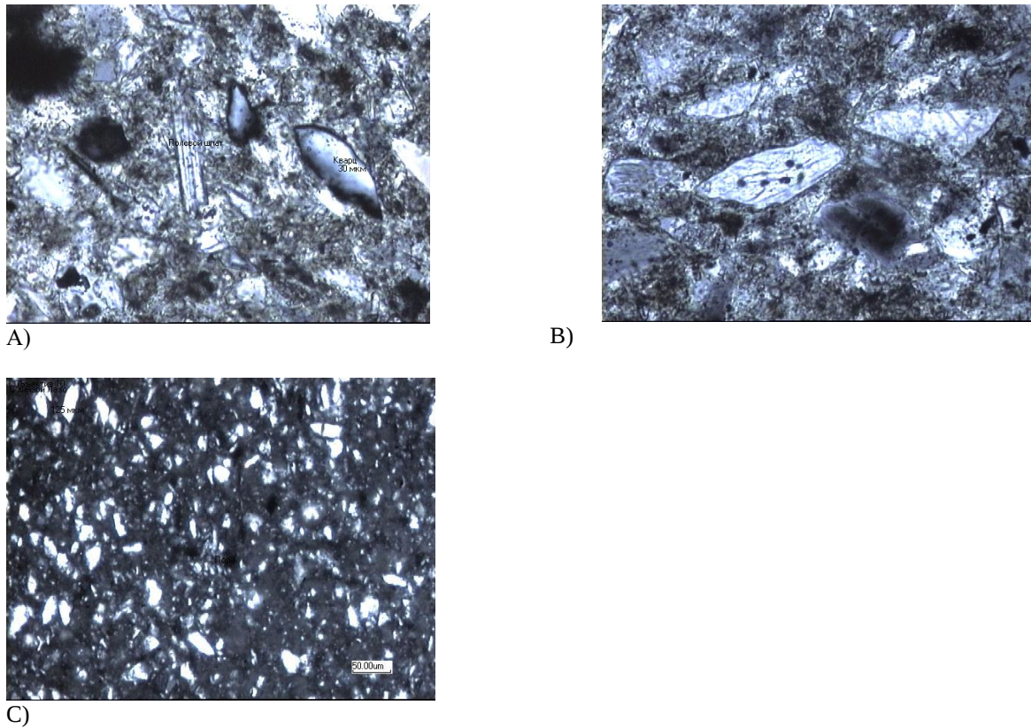
Fig. 3 Micrograph Of Prototypes From Mass S-1, Fired At Temperatures Of 1100, 1200, And 12500c
