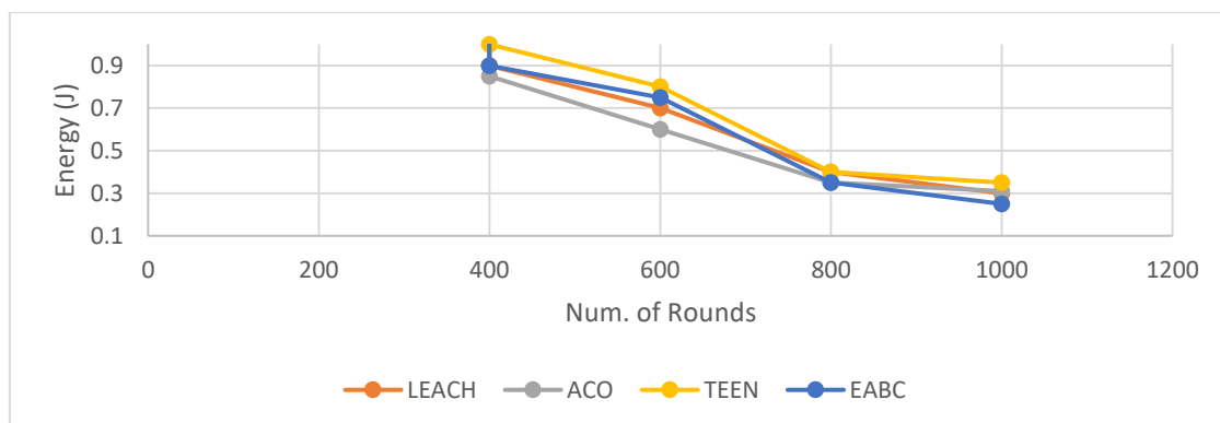
Graph 2: Energy Conservation
