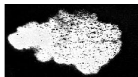
Segmented Image
