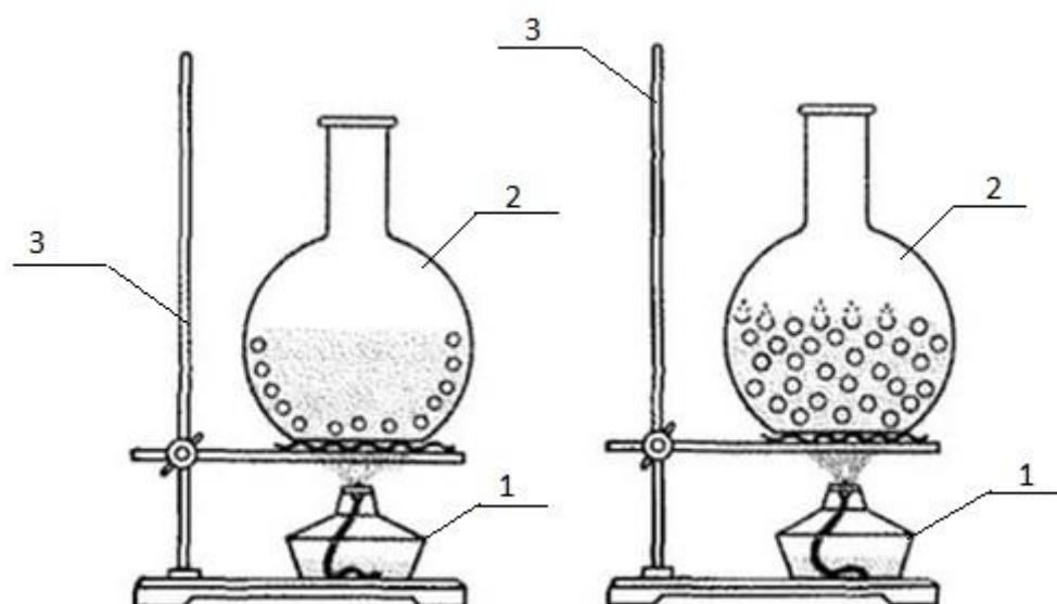
Fig. 1. Diagram of an experimental setup for determining the boiling point
