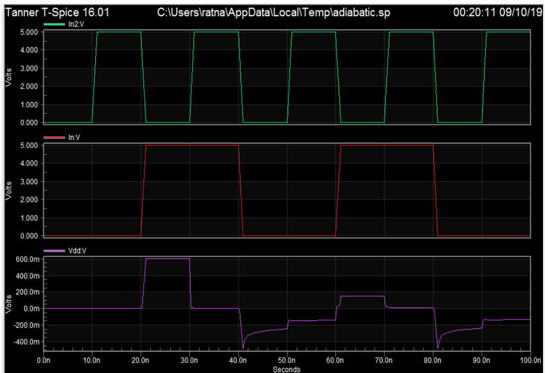
Fig.8 (OUTPUT WAVEFORM)
