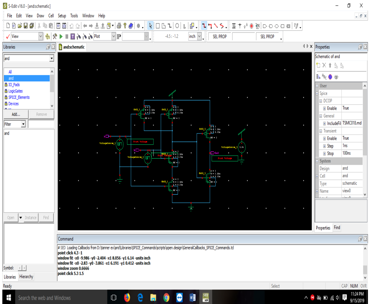
Fig.5 (Schematic of AND gate by fixed CMOS)
