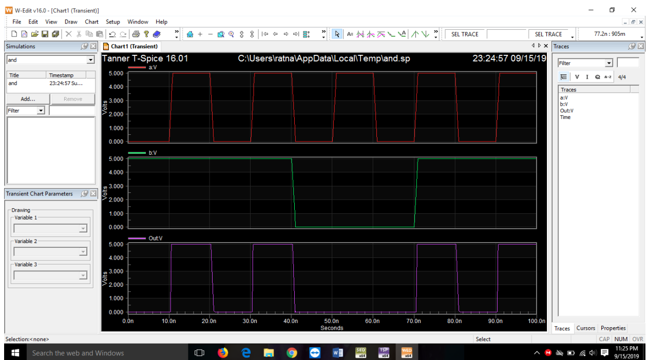
Fig.6 (AND Logic Output)
