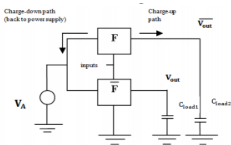
Fig.1. Adiabatic logic
