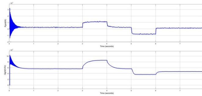
Fig. 8: Grid active and reactive powers for case 4
