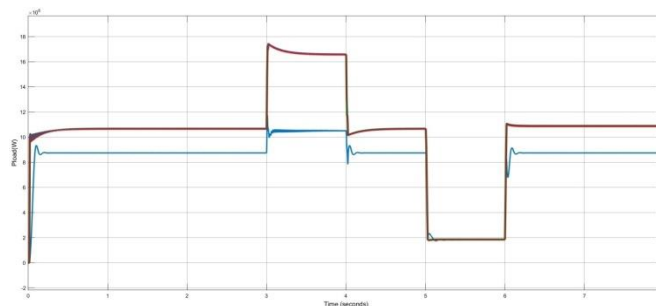
Fig. 7: Active power of load of 4 test systems
