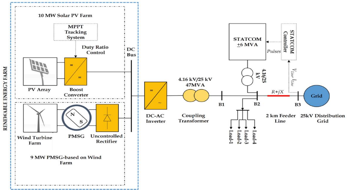
Fig. 1: Proposed distribution test system with RES and STATCOM modules
