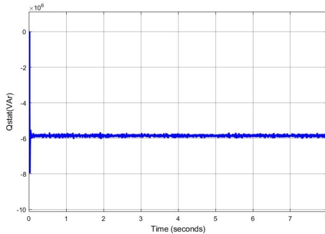
Fig. 11: Reactive power injection from STATCOM with FIS controller
