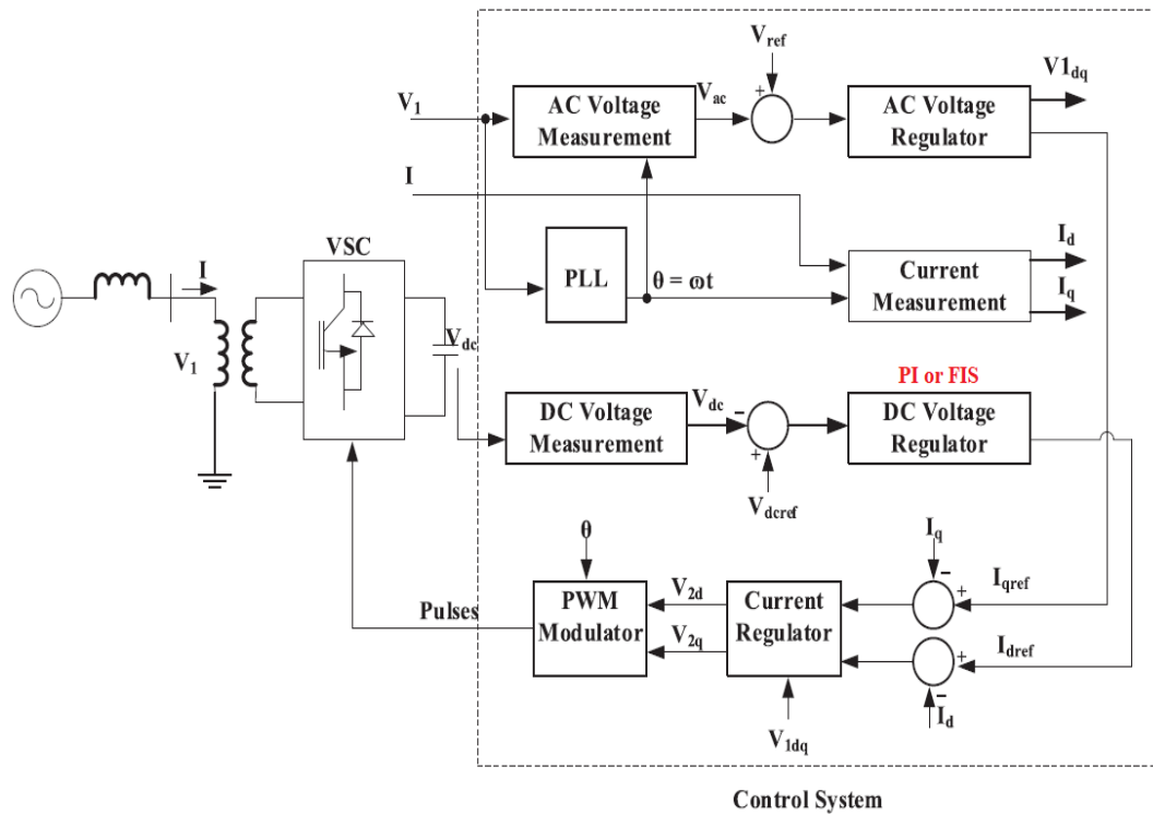
Fig. 5: STATCOM control structure
