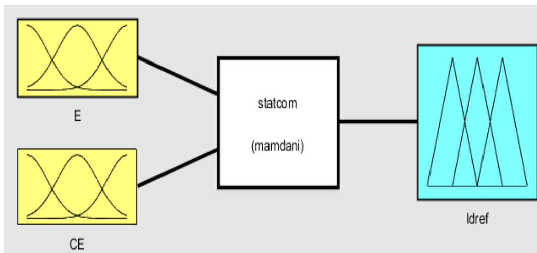
Fig. 6: Fuzzy interface structure for DC voltage regulator
