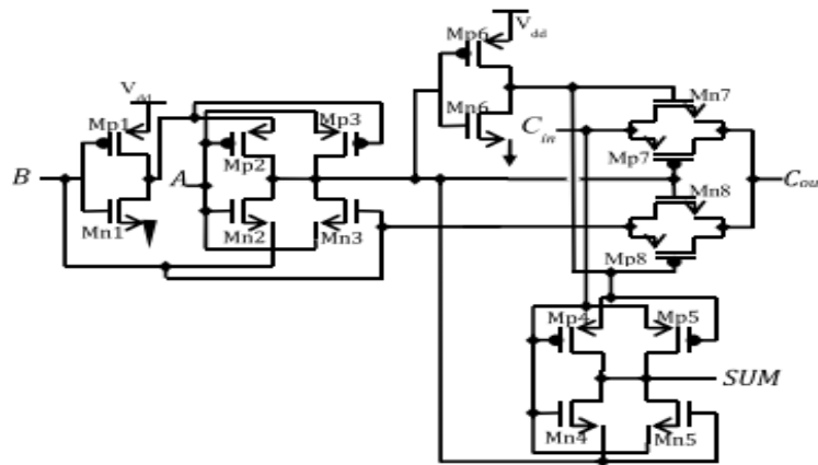
Figure 2.1. Proposed Circuits
