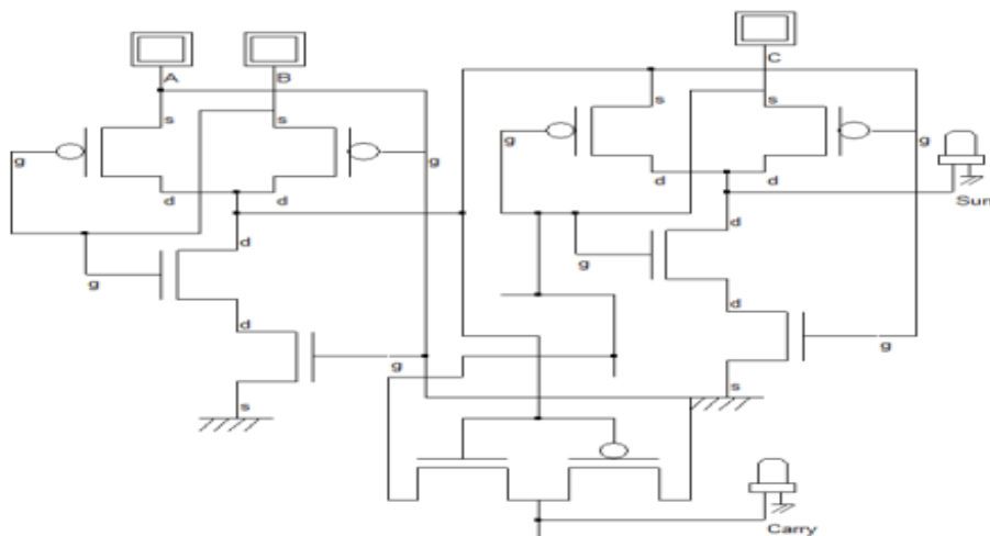
Figure 2.2. Full adder using PTL
