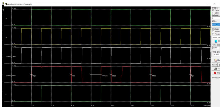
Figure 3.3.Simulation Results
