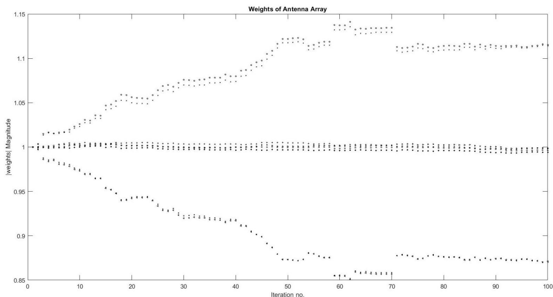
Figure 2. Array Weights of Magnitude (MMSE)
