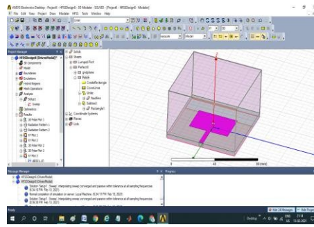
FIGURE 1: Designed slotted patch antenna
