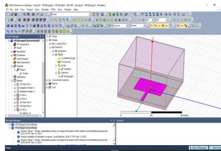
FIGURE 1: Designed slotted patch antenna
