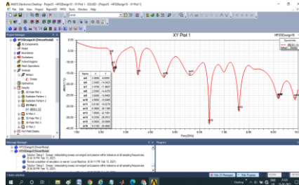
FIGURE 10: Return Loss plot of slotted antenna after first iteration
