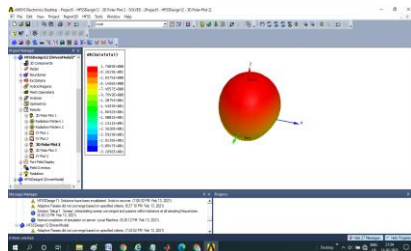
FIGURE 8: Gain of slotted antenna
