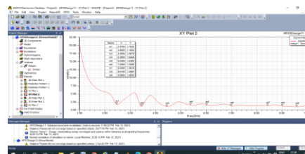
FIGURE 16: VSWR plot of slotted antenna after second iteration
