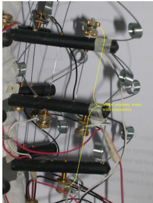
Figure 1.19 SMA wires used as artificial muscles.
