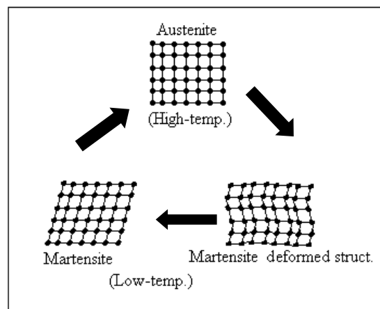
Figure: 1.8 Mechanics of the shape memory effect. (Gilbertson, 2003)
