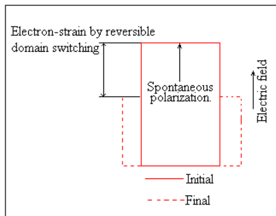
Figure 1.7 Domain switching for electrostrictive polymers. (Adapted Steuer et al, 2006)
