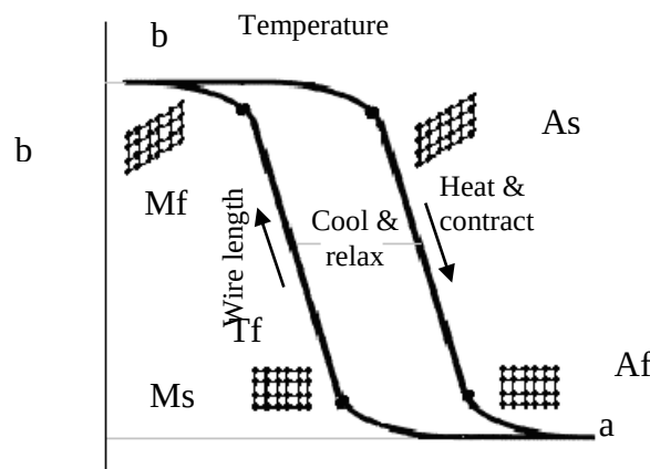
Figure 1.9 Wire lengths vs. Temperature. (Adapted from Gilbertson, 2003)
