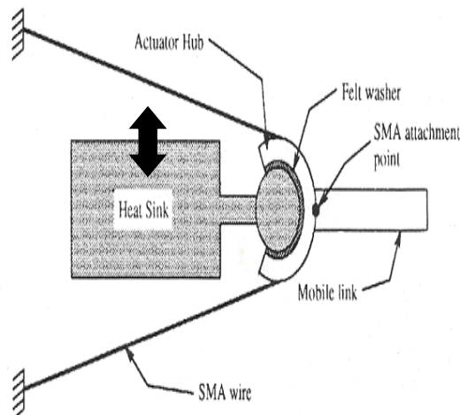
Figure 1.11 Mechanical heat sink (Gorbet and Russell, 1994)
