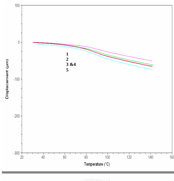
Figure 1.17 DMA test for repeatability in temperature and displacement curves.
