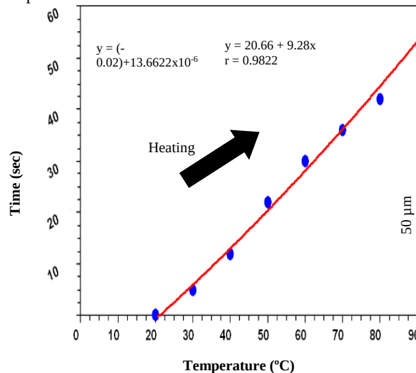
Figure 1.15 Experimental analysis for time of heating SMA wire
