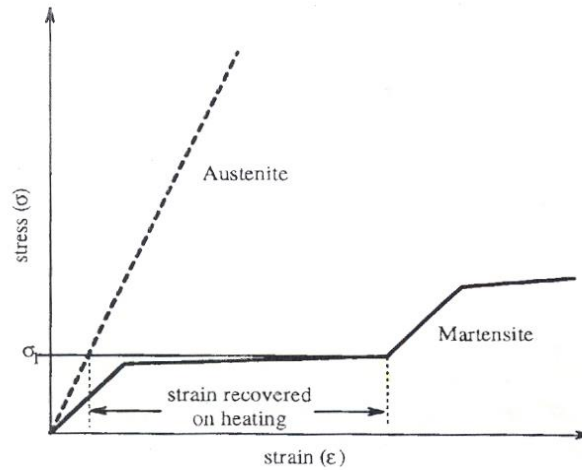
Figure 1.10 Temperature phase for austenite and martensite curves. (Gorbet and Rusell, 1994)
