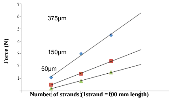
Figure 1.14 Basic properties of different diameter SMA wires
