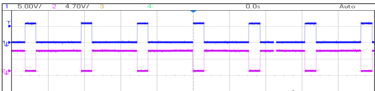
Fig. 8 Complementary Switching Pattern
