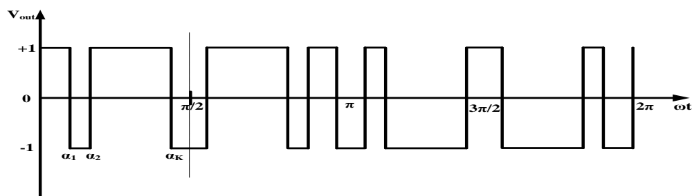
Fig. 1 Bipolar Output voltage waveform
