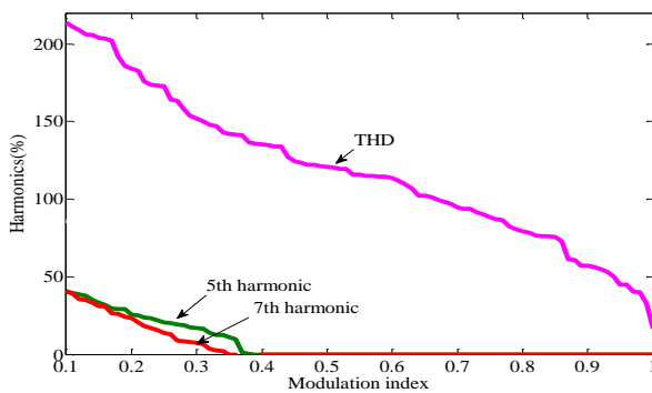
Fig. 4 Harmonic Profile
