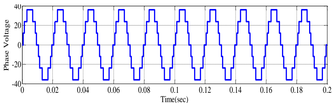
Fig. 9 Experimental Result of Phase output
