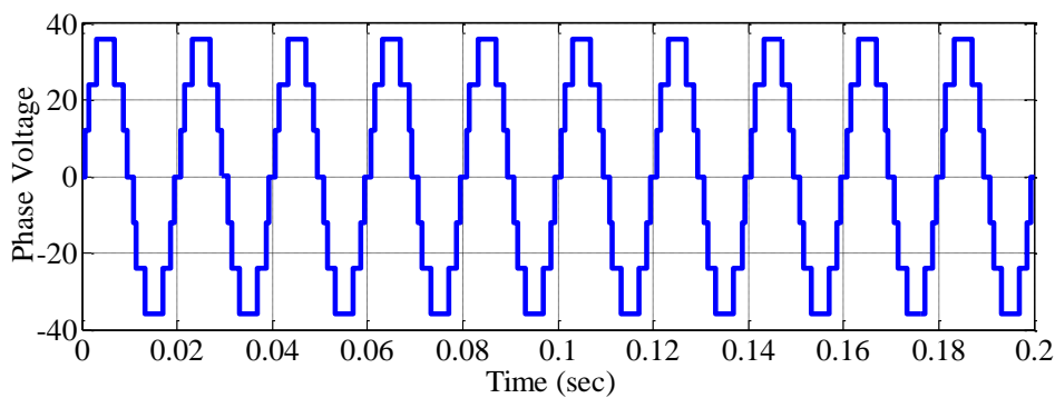
Fig. 3 Output phase voltage
