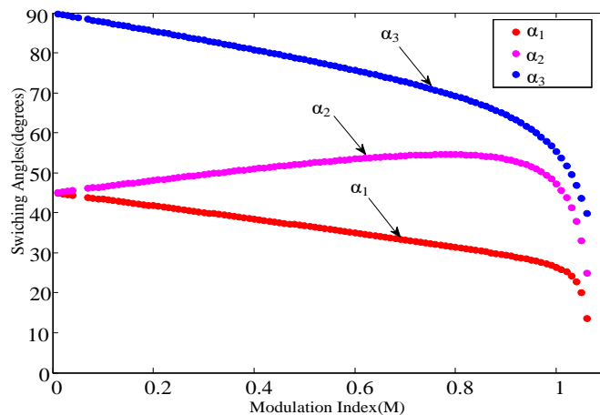
Fig. 2 Variation of switching angles
