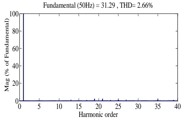
Fig. 5 FFT Analysis
