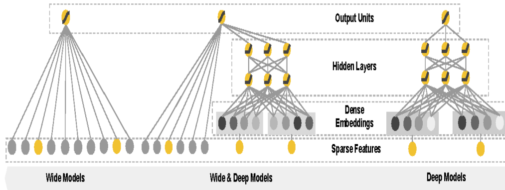
Fig 2: The spectrum of Wide &amp; Deep models.
