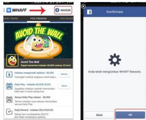
Figure 1. Whaff interface
