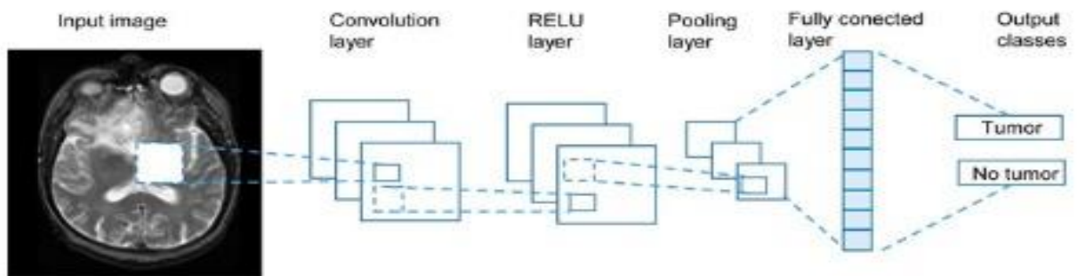
Fig. 1. Convolutional Neural Network work
