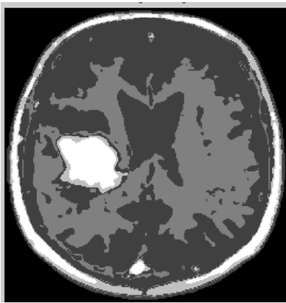
Fig. 7 Enhanced Image
