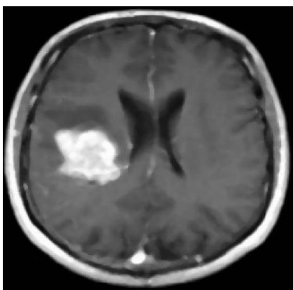
Fig.5 Input Image
