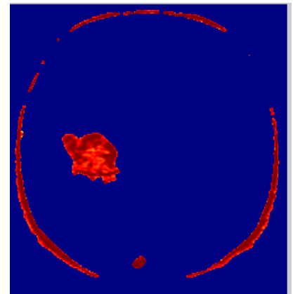
Fig. 9 Extract Tumor
