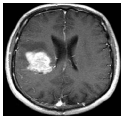
Fig.8 Segmented Image
