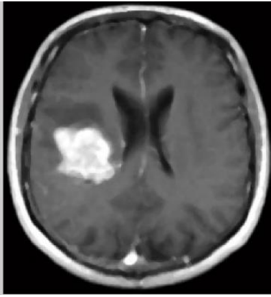
Fig. 6 Filtered Image
