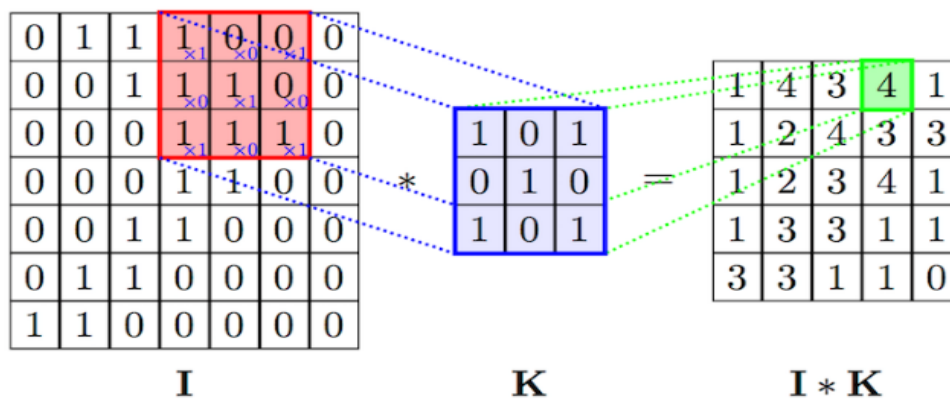
Fig 2. Convolutional layer
