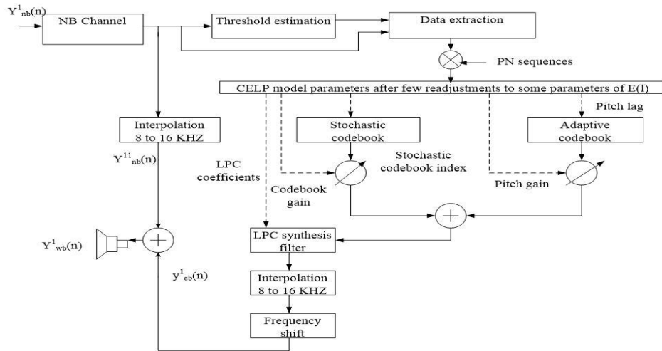
Figure 2: Proposed receiver
