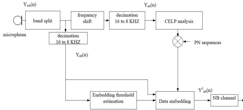
Figure 1: Proposed transmitter
