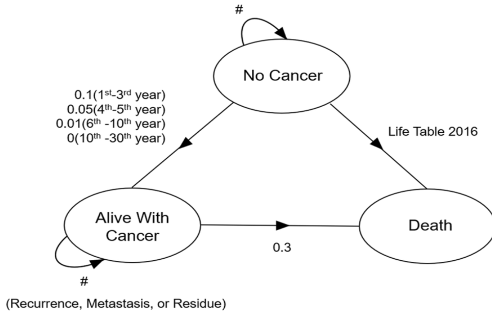
Figure 2. Proposed Bayesian model transition diagram
