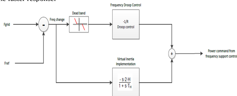
Figure 3: Inverter dynamic with Virtual Inertia
