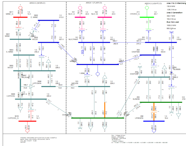
Figure 4: Sample test system
