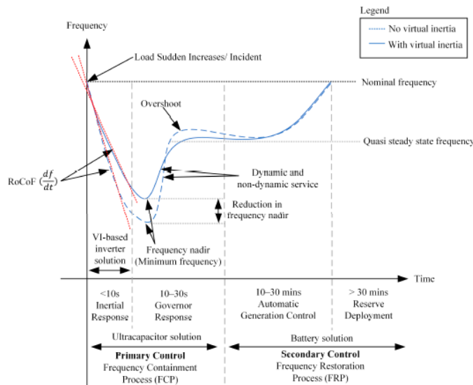
Figure 2: The effect of Virtual Inertia in low inertia system
