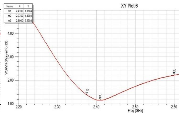
Fig.1.17 - VSWR of 1 x 4 Array with DGS
