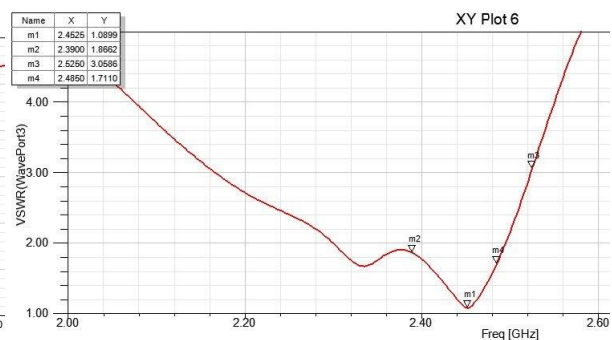
Fig.1.12- VSWR of 1 x 4 MSPA Array
