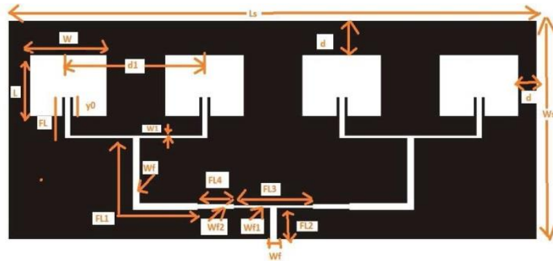
Fig.1.9– 1 x 4 microstrip array antenna
