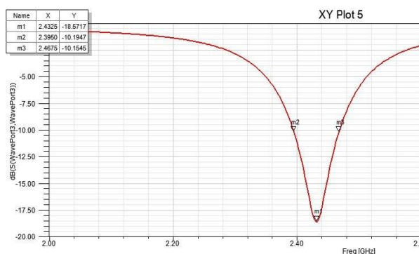
Fig. 1.4 - Return Loss for single patch Antenna.
