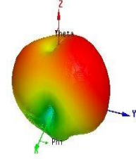
Fig.1.19- 3 D Polar Plot of 1 x 4 Array with DGS
