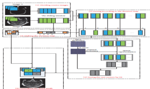
Figure 1: The framework of the image fusion method based on sparse representation and feature extraction.
