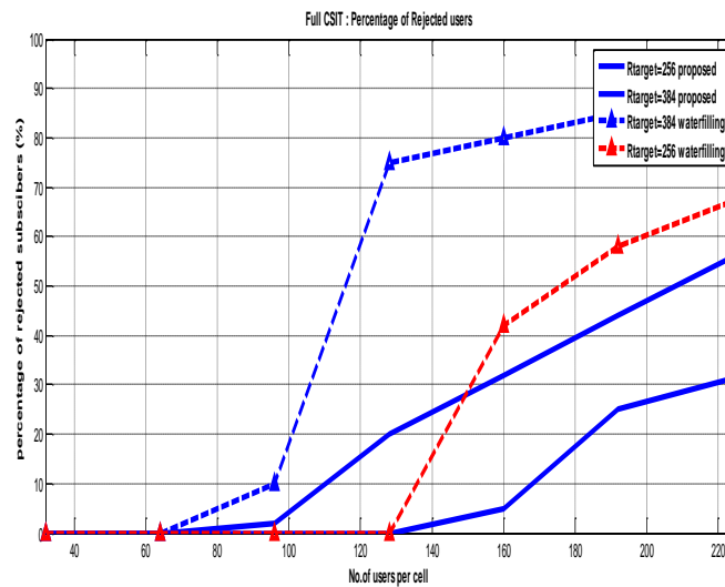
Fig.2. Percentage of rejected users for Full-CSIT,
