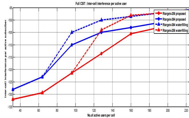
Fig.4: Inter-cell Interference per Active sub-carriers for Full-CSIT.
