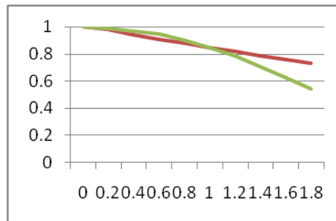
Figure 1. Reliability (Exponential and Weibull distribution) vs time
