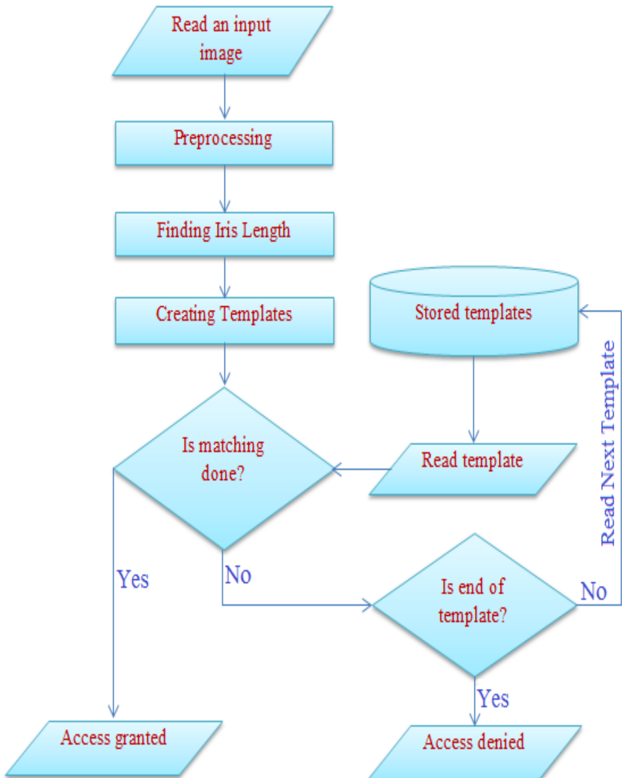
Fig 5.2: Work flow for feature matching
