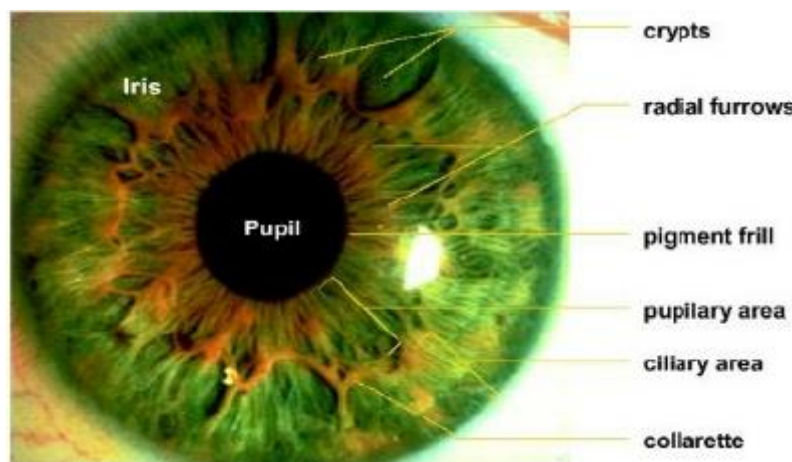
Fig 1.1: Structure of an Iris
