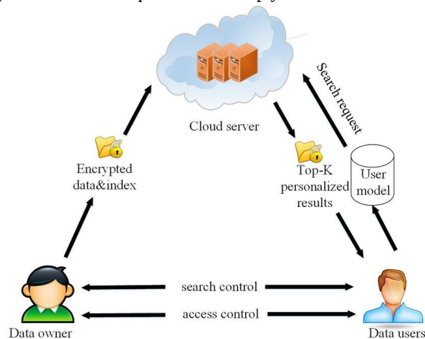
Figure. 1 Architecture of the search through encrypted data on cloud
