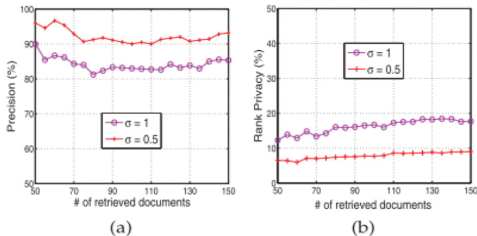
Figure.2 There is a discrepancy among (a) precision also (b) rank privacy with a particular selection of the standard deviation for the random variables.
