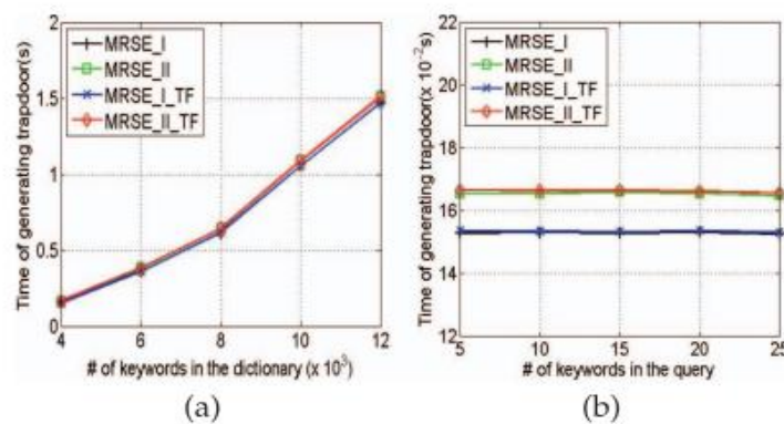
Figure 4. Trapdoor processing period bill (a) Keywords in different dictionary sizes with the same question. (b) For different question keyword numbers in the same dictionary
