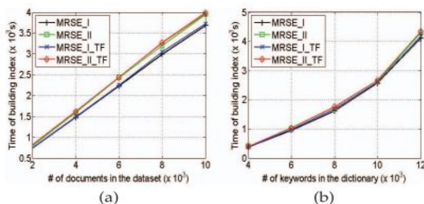
Figure. 3 The time cost of building index. (a) For the different size of the data set with the same dictionary, (b) For the same data set with different size of the dictionary
