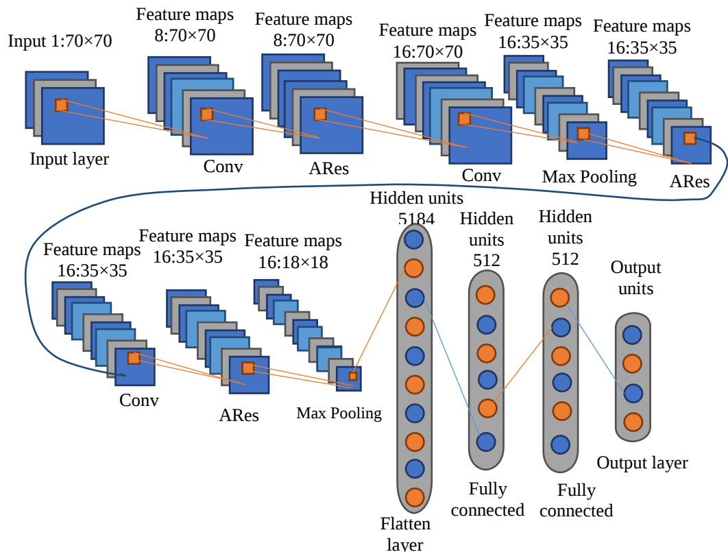
Fig.2.The EMiCoAReNet framework
