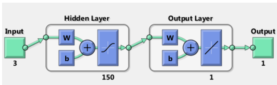
Fig.7 Net radiation 2018-2019 model
