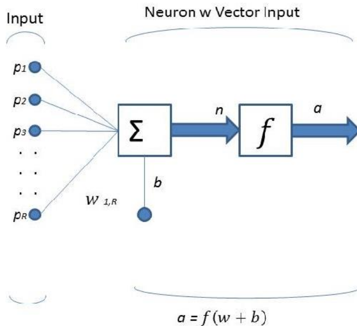
Fig.1 Simplified flow chart of artificial neural network
