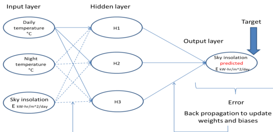
Fig.5 Work scheme #1. Input: Daily temperature, night temperature and solar sky insolation. Output-solar insolation
