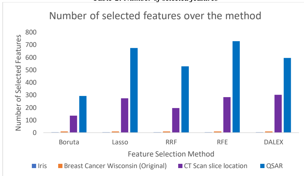
Figure-2: Number of selected features over the methods
