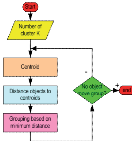
Fig. 5. K-means iteration
