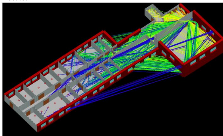
Fig. 2. The signal beam tracing method of calculation
