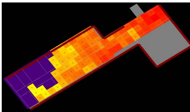
Fig. 4. The distribution level Wi-Fi hotspot signal Wireless Insite environment
