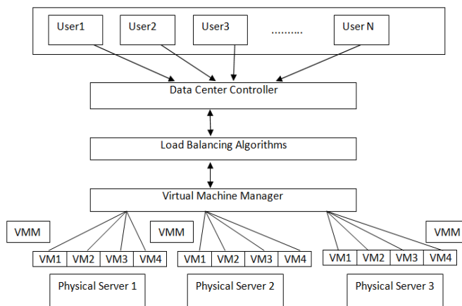
Fig 1. Load Balancing Model
