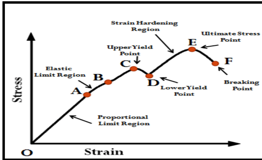
Figure 1: Stress-Strain Relationship for Mild Steel or Ductile Material
