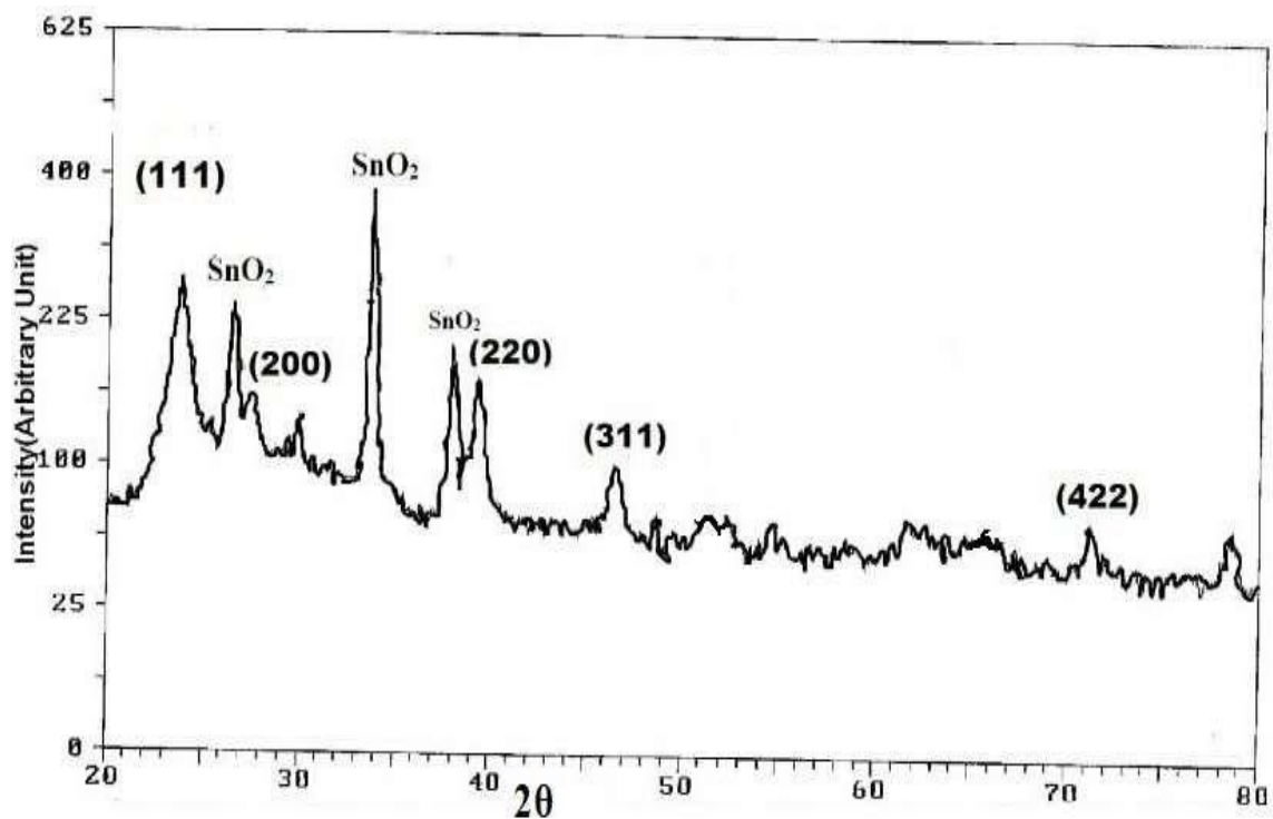
Fig 4. X-Ray diffraction pattern of a CdHgTe film grown at -700 mV w.r.t. SC electrode grown from the bath of composition X=0.2.
