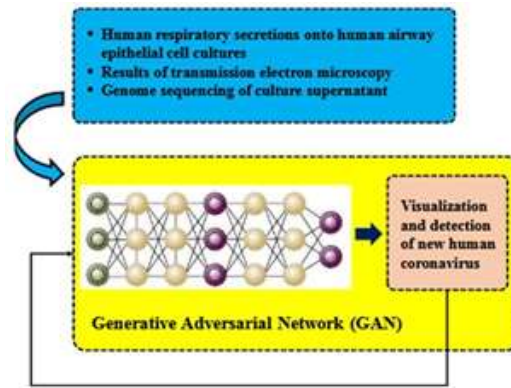
Fig2:GANnetwork
