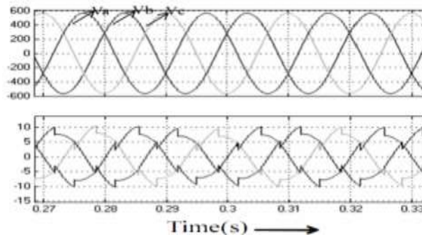
Fig.3: Instantaneous Value of Grid voltage and current for Grid connected system with non-linear loads
