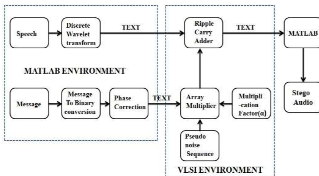
Figure 1: Proposed DWT based Speech Steganography.
