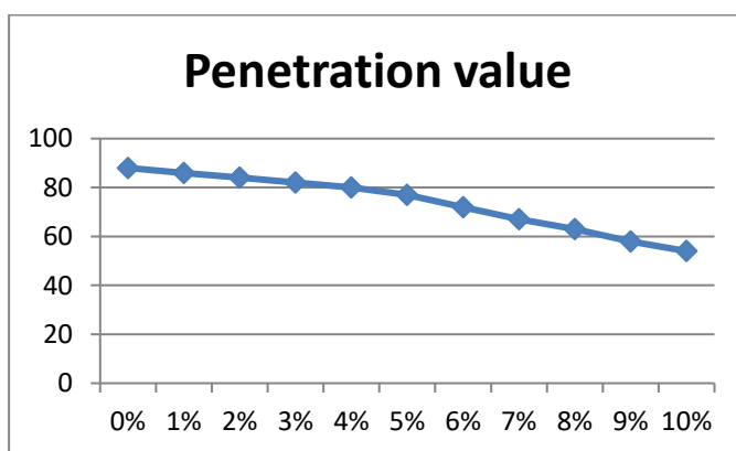
Penetration value v/s Waste Plastic content
