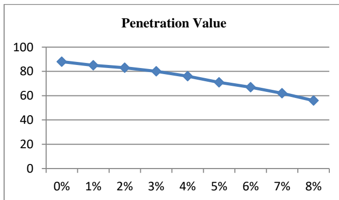
Penetration value v/s Lignin content
