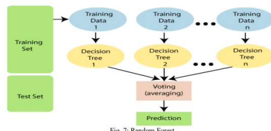
Fig. 7: Random Forest
