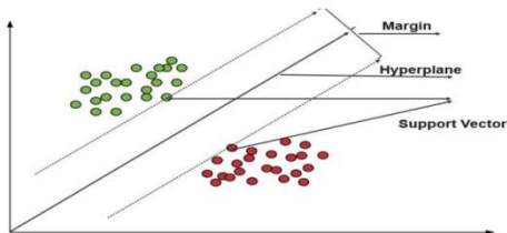
FIG 8: SVM
