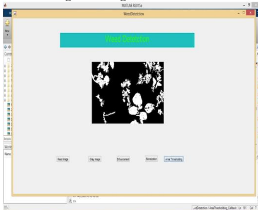
Fig 11: Area Thresholding.
