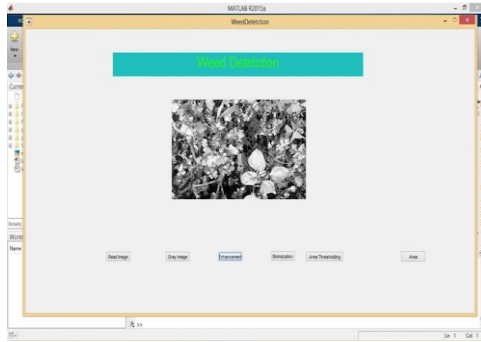
Fig 9: Image Enhancement.
