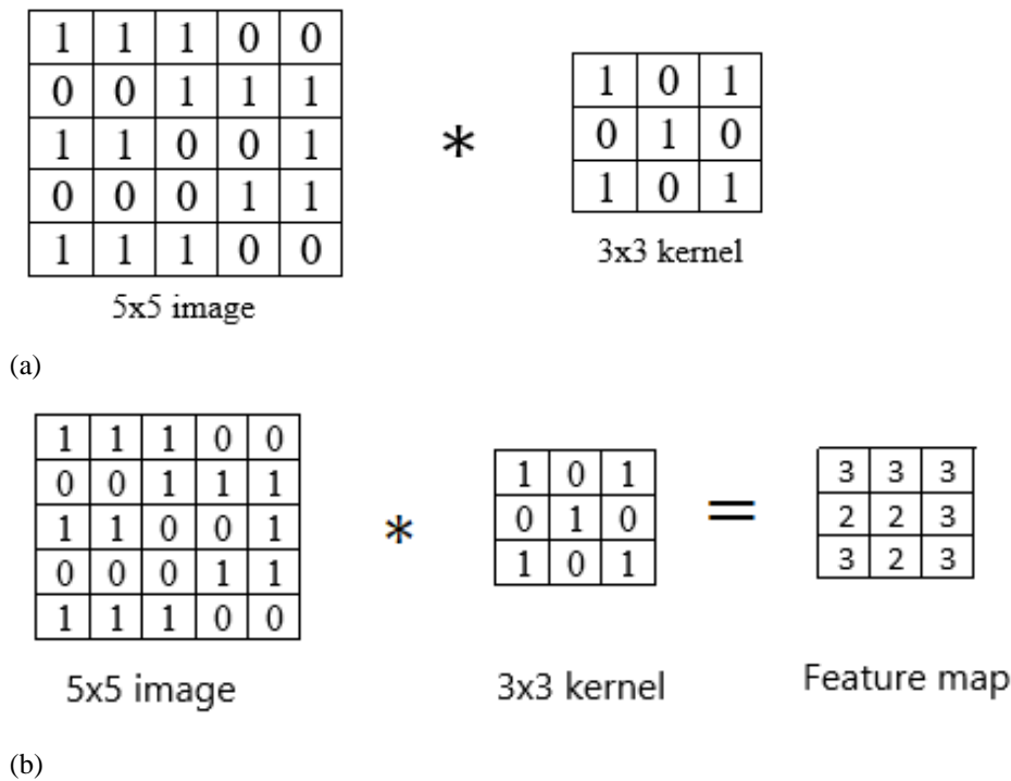
Fig. 3: Example of convolution layer process (a) an image with size 5x5 is convolving with 3x3 kernel (b) Convolved feature map.
