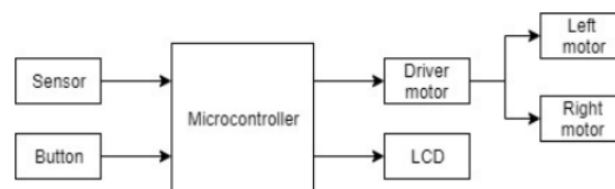
Fig. 1. Robot system block diagram
