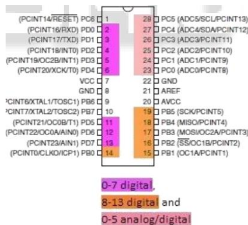
Fig. 5: Pin Diagram of Atmega328P
