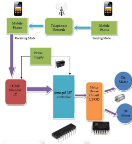
Fig. 1: Block Diagram of DTMF based Navigation Mobile Robot
