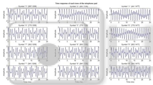
Fig. 3: DTMF Tone Frequency
