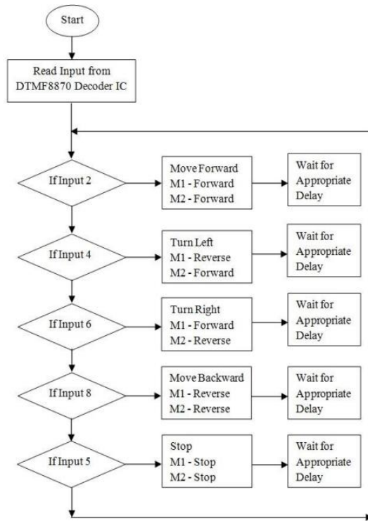
Fig. 9: Flow diagram of system
