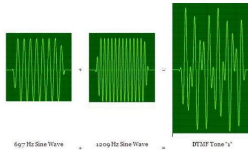
Fig. 2: Two Pure Sine Waves combine for form the DTMF Tone for "1"[3]
