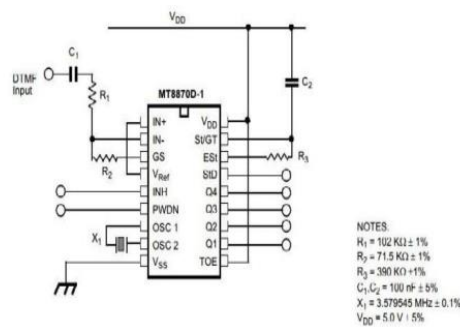
Fig. 4: MT-8870 DTMF Decoder Configuration [4]
