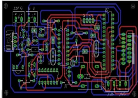
Fig. 11: Printed Circuit Board for DTMF based Controlled Robot
