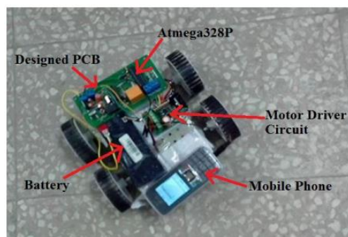
Fig. 12: Designed Robot
