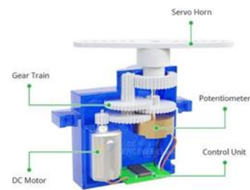
Fig .5: Servomotor
