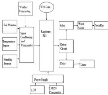
Fig 16. Block diagram
