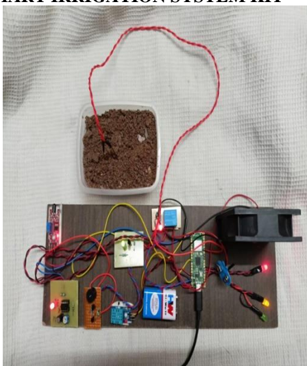
Fig 17 Smart Irrigation system Kit
