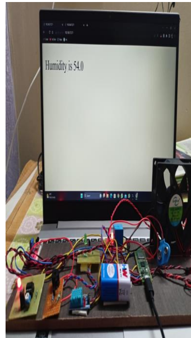
Fig 19 Humidity Output
