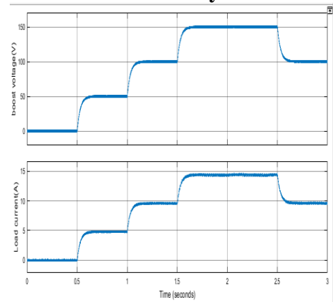
Fig.8. BOOST CONVERTER STEP REFERENCE without fuzzy
