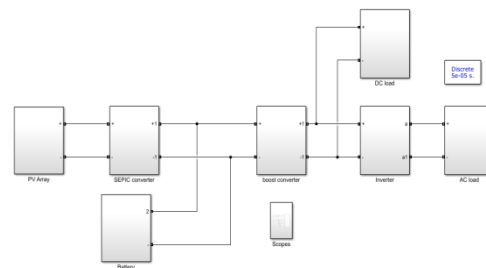
Fig.2. Simulation circuit
