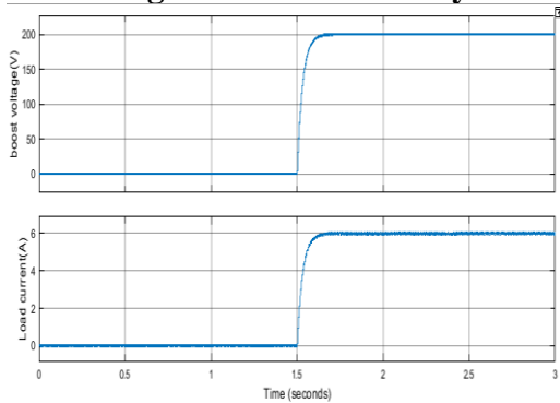
Fig.5. MPPT with fuzzy
