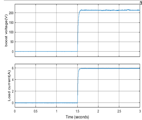
Fig.7. BOOST CONVERTER using with fuzzy
