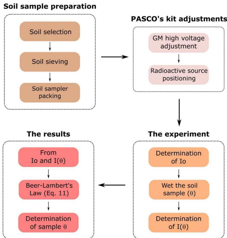
Figure 4. Flow chart of the steps followed for the soil water content ( \theta ) measurement using the simplified gamma-ray attenuation method. GM: Geiger-Müller detector. I _0 : Intensity of the incident photon beam. I: Intensity of the transmitted photon beam.
