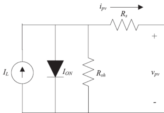
Fig. Equivalent circuit diagram of the PV cell
