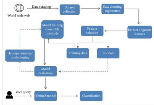
Fig.1: Workflow diagram
